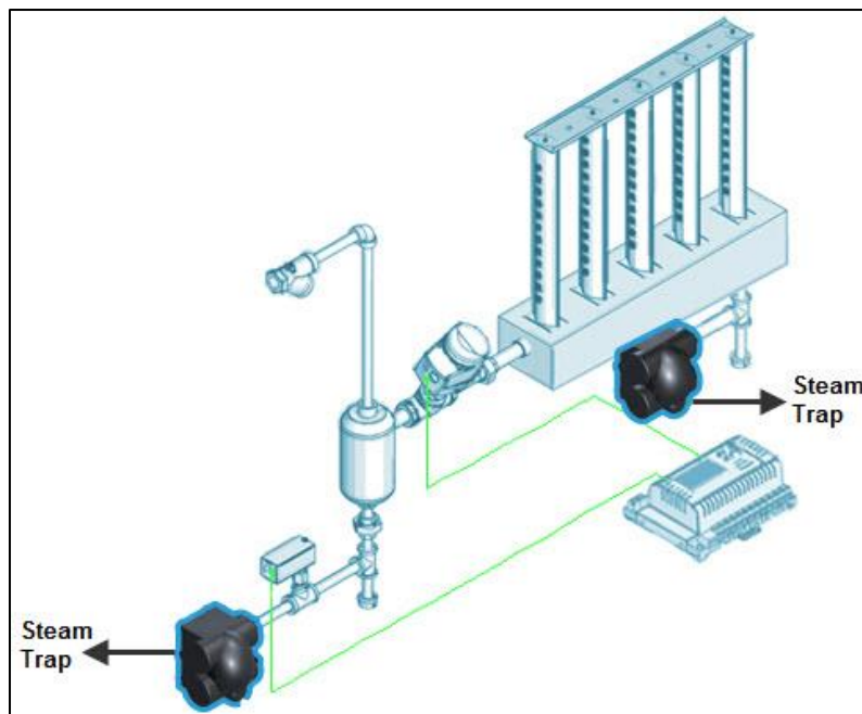
Illustration 15 - Float and Thermostatic Steam Trap Installation
