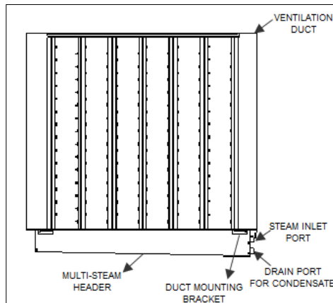
Illustration 6 - Manifold Installation: Side View
