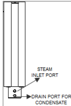
Illustration 5 - Manifold Installation: Front View
