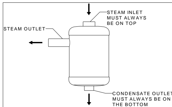
Illustration 12 - Correct Installation
