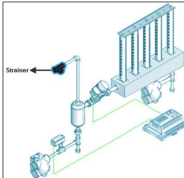
Illustration 17 - Strainer Installation
